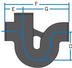
RUNNING TRAP (with 4” single vent)
