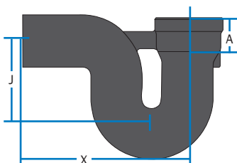
“P” TRAP WITH ½” HEEL TAP
