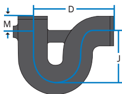
“P” TRAP (with ½" tap primer)
