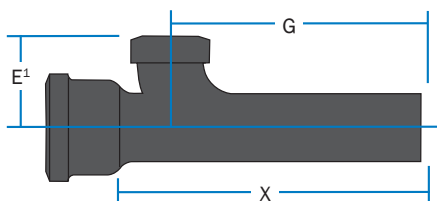
LONG SANITARY TAPPED TEE
